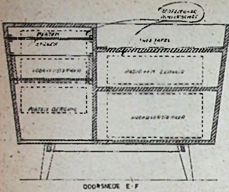
DOORSNED E-F
